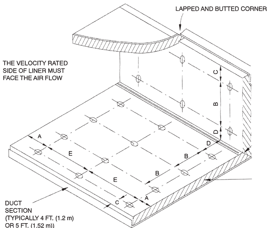
Maximum fastener spacing
