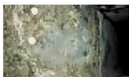
Result w/ Fibrous: Mold growth on insulation
